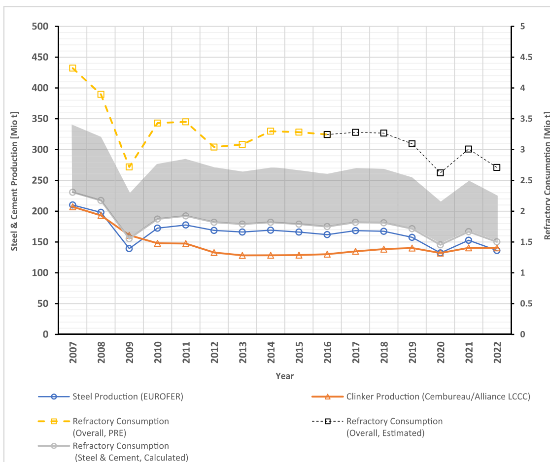
Fig. 1. Development of EU steel and cement production and refractory consumption with time. Refractory consumption in 2022 can be estimated at 2.7 Mt, with 1.36 Mt being attributed to steel and 0.14 Mt to cement clinker production.
